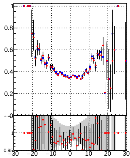
—•— DQM_TT_mkFit-DQM_original —•— DQM_TT_mkFit-DQM_modified4
