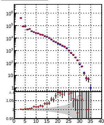
DQM_TT_mkFit-DQM_original DQM_TT_mkFit-DQM_modified4
