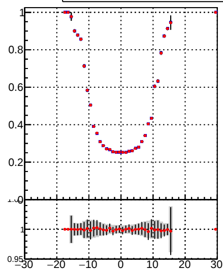
—•— DQM_TT_mkFit-DQM_original —•— DQM_TT_mkFit-DQM_modified4
