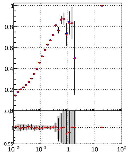
—•— DQM_TT_mkFit-DQM_original —•— DQM_TT_mkFit-DQM_modified4
