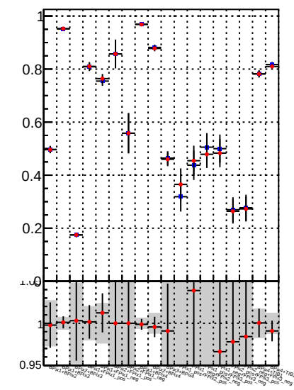
Fake rate vs. — DQM_TT_mkFit-DQM_original — DQM_TT_mkFit-DQM_modified4
