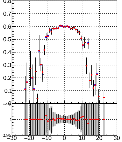
Efficiency vs. sim PV z Legend: DQM_TT_mkFit-DQM_original (blue line with markers) DQM_TT_mkFit-DQM_modified4 (red line with markers)
