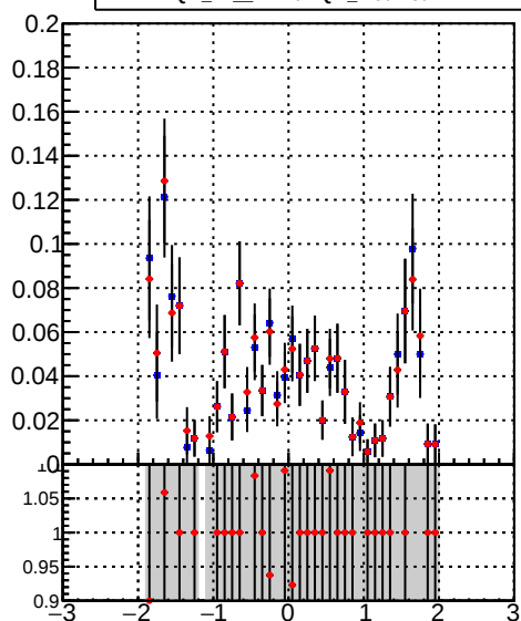
—•— DQM_TT_mkFit-DQM_original —•— DQM_TT_mkFit-DQM_modified4
