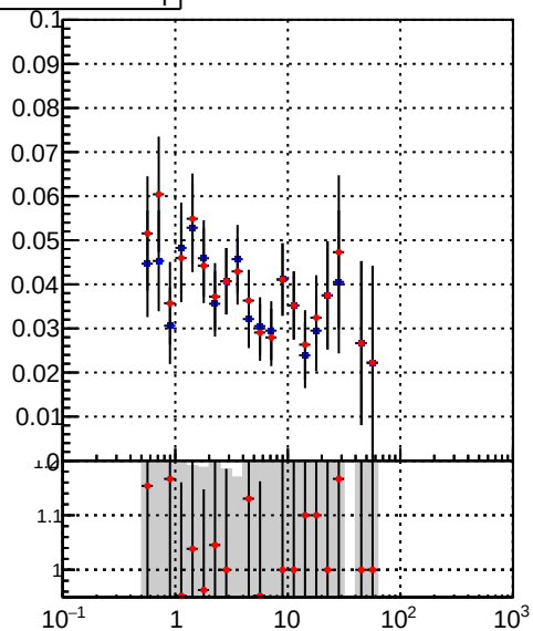
—●— DQM_TT_mkFit-DQM_original —●— DQM_TT_mkFit-DQM_modified4
