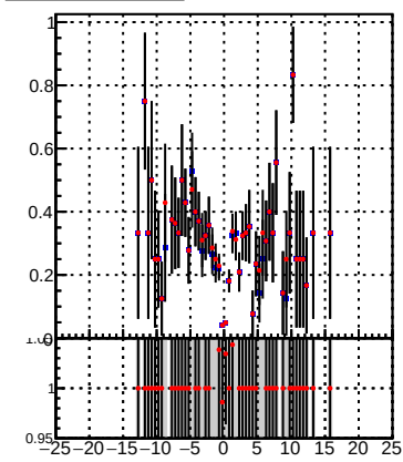
Efficiency vs Dxy(PV) Legend: DQM_TT_mkFit-DQM_original DQM_TT_mkFit-DQM_modified4
