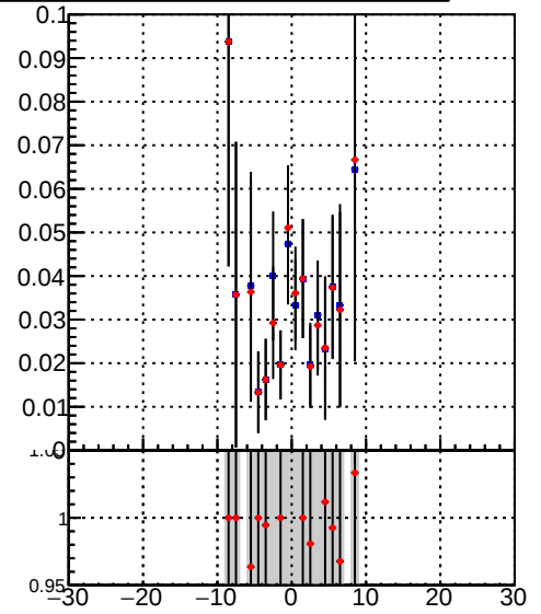
Efficiency vs vertpos Legend: DQM_TT_mkFit-DQM_original (blue dots) DQM_TT_mkFit-DQM_modified4 (red dots)
