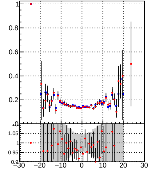
Efficiency vs. sim PV z Legend: DQM_TT_mkFit-DQM_original (blue line with error bars) DQM_TT_mkFit-DQM_modified4 (red line with error bars)
