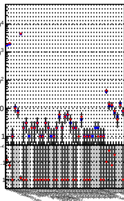
N of reco track vs. \chi^2
