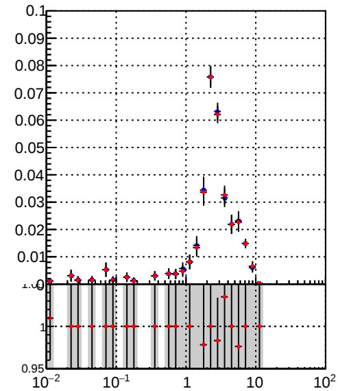
Efficiency vs. vertpos Legend: DQM_TT_mkFit-DQM_original (Blue line with markers) DQM_TT_mkFit-DQM_modified4 (Red line with markers)
