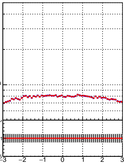
N of simulated tracks vs phi
