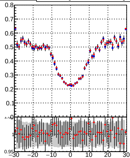
—•— DQM_TT_mkFit-DQM_original —•— DQM_TT_mkFit-DQM_modified4
