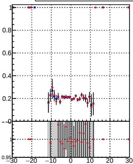
■ DQM_TT_mkFit-DQM_original ● DQM_TT_mkFit-DQM_modified4
