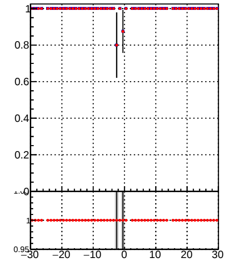
Fake rate vs vertpos Legend: DQM_TT_mkFit-DQM_original (black line) DQM_TT_mkFit-DQM_modified4 (red line)
