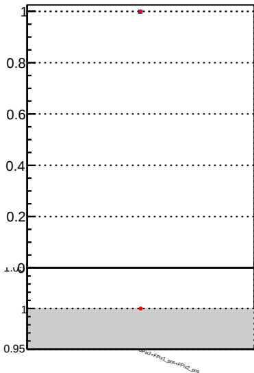
Fake rate vs. — DQM_TT_mkFit-DQM_original — DQM_TT_mkFit-DQM_modified4
