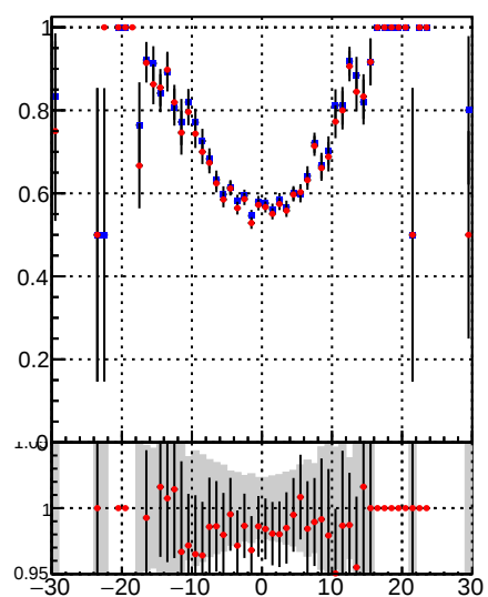
Fake rate vs d —●— DQM_{TT} mkFit-DQM_original —●— DQM_{TT} mkFit-DQM_modified4
