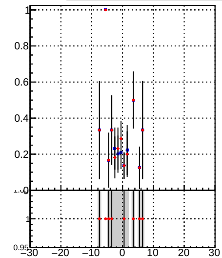
—•— DQM_TT_mkFit-DQM_original —•— DQM_TT_mkFit-DQM_modified4
