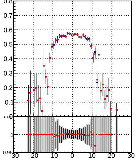
Efficiency vs. sim PV z Legend: DQM_TT_mkFit-DQM_original (blue line) DQM_TT_mkFit-DQM_modified4 (red line)
