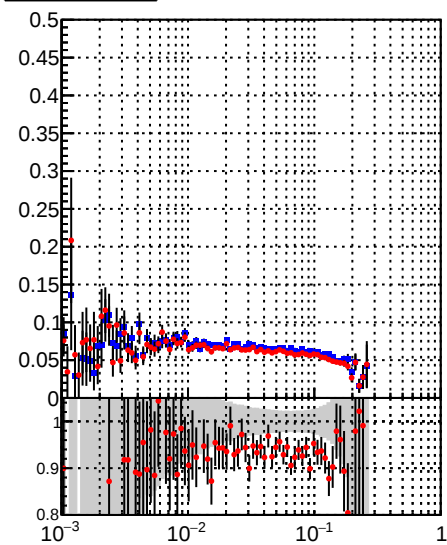
—•— DQM_TT_mkFit-DQM_original —•— DQM_TT_mkFit-DQM_modified4
