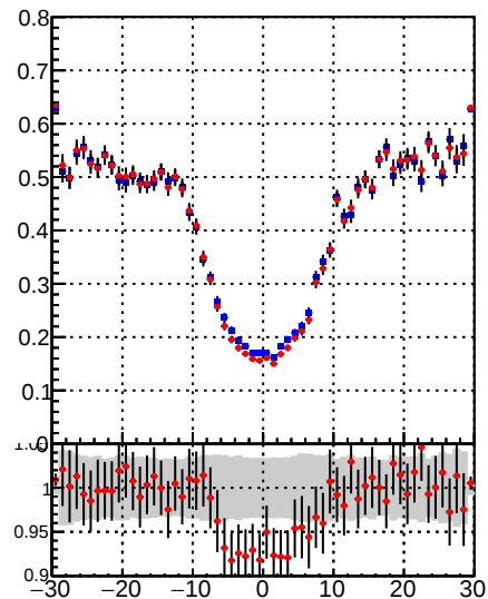
—●— DQM_TT_mkFit-DQM_original —●— DQM_TT_mkFit-DQM_modified4
