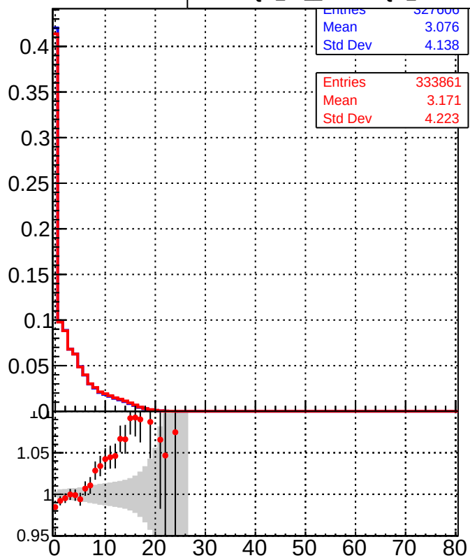
—■— DQM_TT_mkFit-DQM_original —●— DQM_TT_mkFit-DQM_modified4
