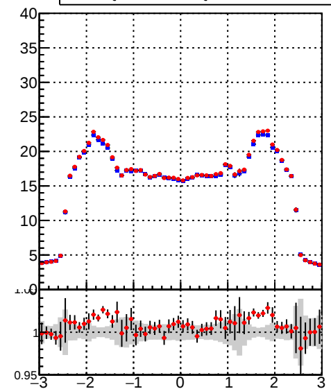
mean hit Legend: DQM_TT_mkFit-DQM_original (blue line), DQM_TT_mkFit-DQM_modified4 (red line)
