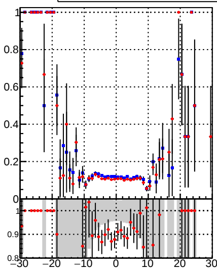
■ DQM_TT_mkFit-DQM_original ■ DQM_TT_mkFit-DQM_modified4
