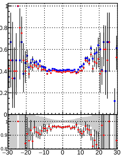
Fake rate vs d —●— DQM TT mkFit-DQM_original —●— DQM TT mkFit-DQM_modified4
