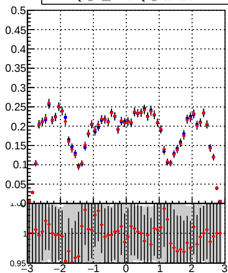
DQM_TT_mkFit-DQM_original DQM_TT_mkFit-DQM_modified3
