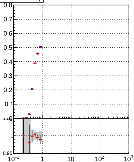
DQM_TT_mkFit-DQM_original DQM_TT_mkFit-DQM_modified3
