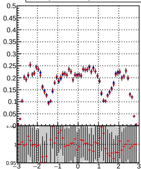
DQM_TT_mkFit-DQM_original DQM_TT_mkFit-DQM_modified3
