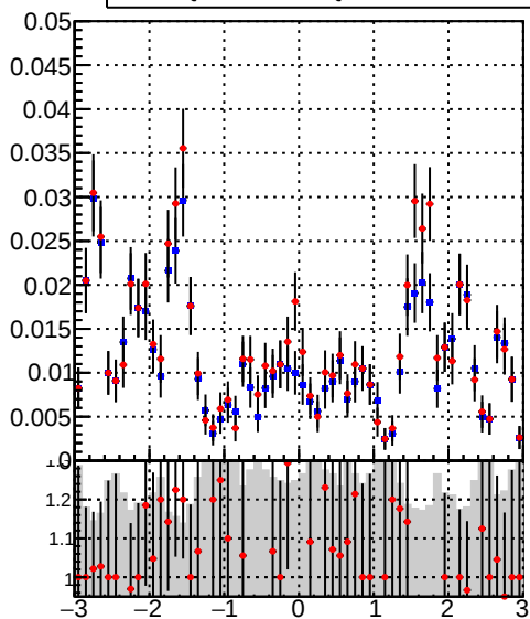
— DQM_TT_mkFit-DQM_original — DQM_TT_mkFit-DQM_modified3
