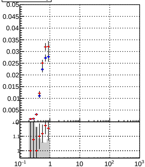
— DQM_TT_mkFit-DQM_original — DQM_TT_mkFit-DQM_modified3
