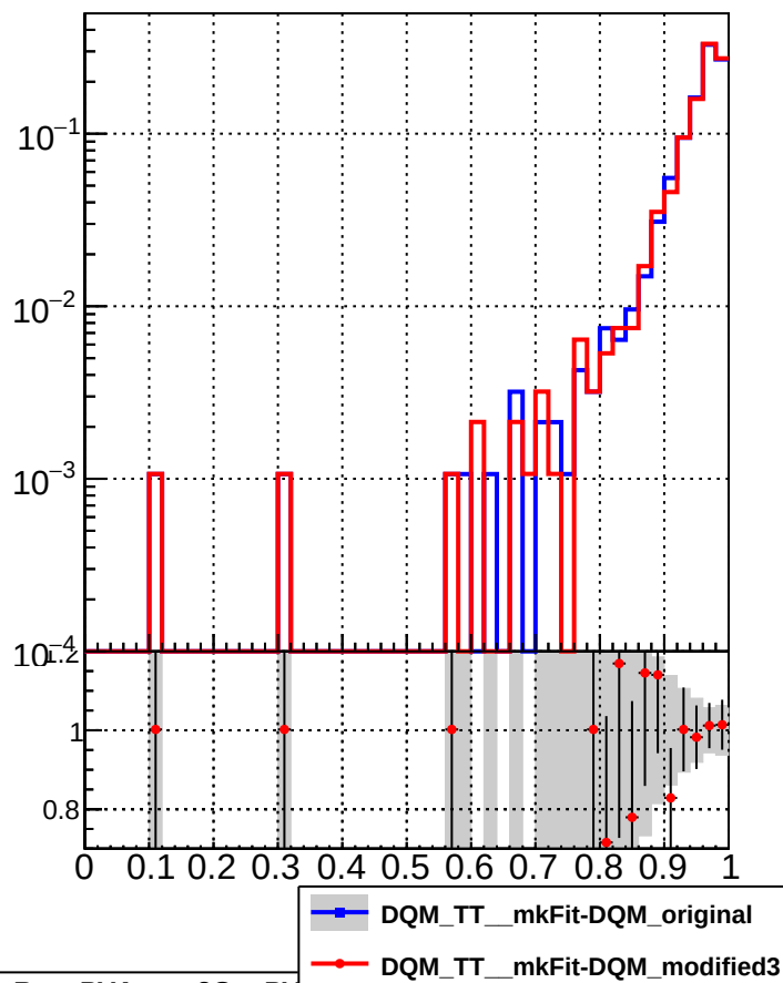
RecoPVAssoc2GenPVMatched_Missing
