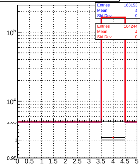
mean hit Legend: DQM_TT_mkFit-DQM_original (blue line), DQM_TT_mkFit-DQM_modified3 (red line)
