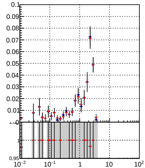
Efficiency vs vertpos — DQM_TT_mkFit-DQM_original — DQM_TT_mkFit-DQM_modified3
