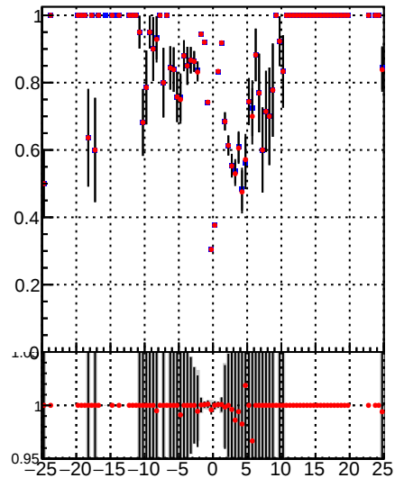
—●— DQM_TT_mkFit-DQM_original —●— DQM_TT_mkFit-DQM_modified3
