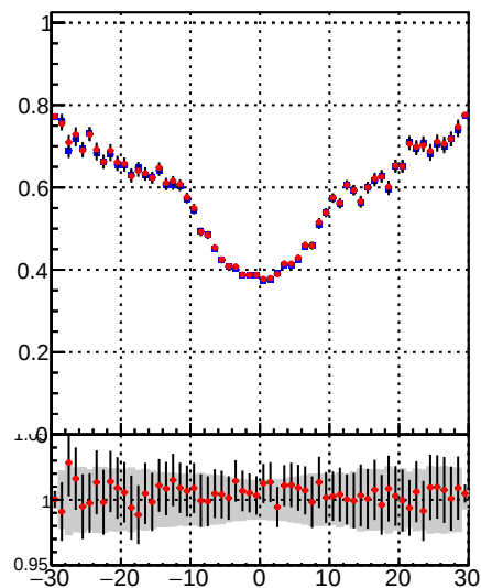
—●— DQM_TT_mkFit-DQM_original —●— DQM_TT_mkFit-DQM_modified3
