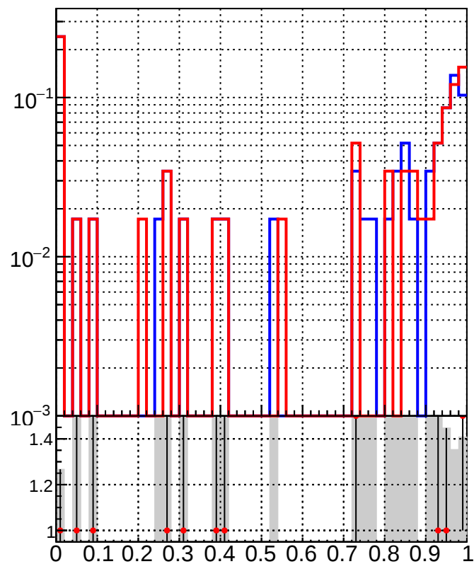
RecoPVAssoc2GenPVNotMatched_Purity
