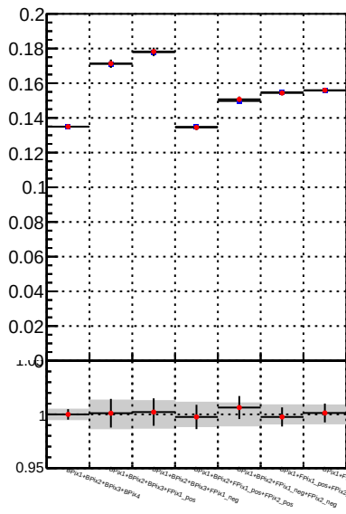
Fake rate vs. —●— DQM TT mkFit-DQM_original —●— DQM TT mkFit-DQM_modified3
