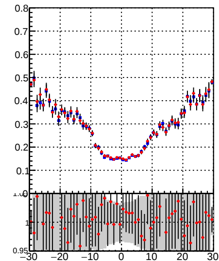
—●— DQM_TT_mkFit-DQM_original —●— DQM_TT_mkFit-DQM_modified3
