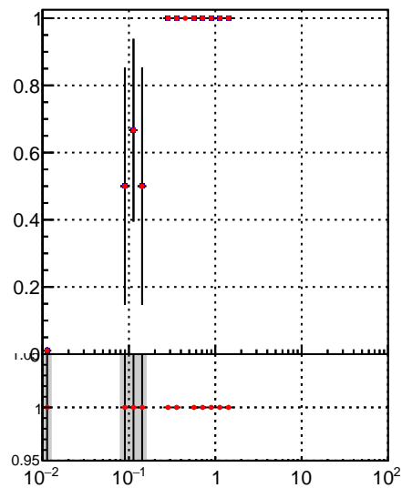
Fake rate vs v ■ DQM_TT_mkFit-DQM_original ● DQM_TT_mkFit-DQM_modified3
