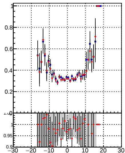
—●— DQM_TT_mkFit-DQM_original —●— DQM_TT_mkFit-DQM_modified3
