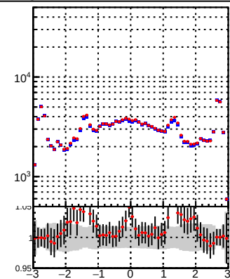
it-DQM_original it-DQM_modified3
