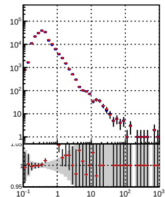
it-DQM_original it-DQM_modified3
