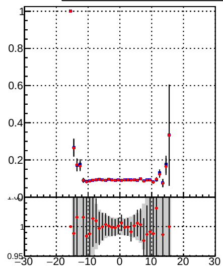
■ DQM_TT_mkFit-DQM_original ● DQM_TT_mkFit-DQM_modified3
