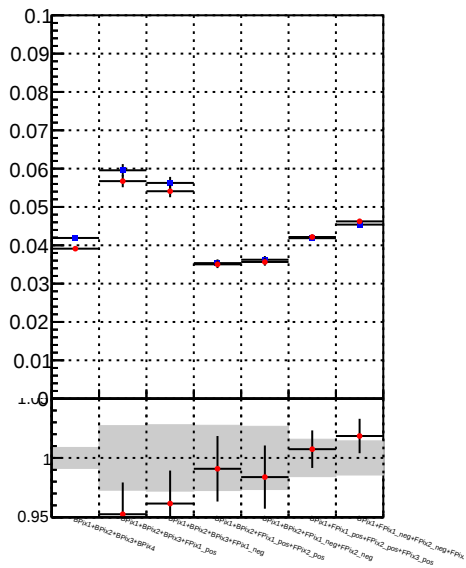
Fake rate vs. —•— DQM TT mkFit-DQM_original —•— DQM TT mkFit-DQM_modified3
