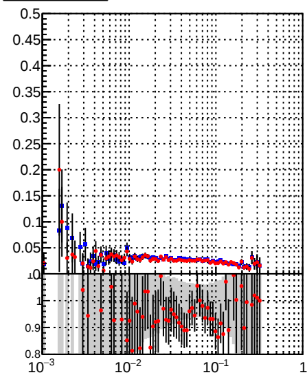
Fake rate vs \epsilon DQM_TT_mkFit-DQM_original DQM_TT_mkFit-DQM_modified3
