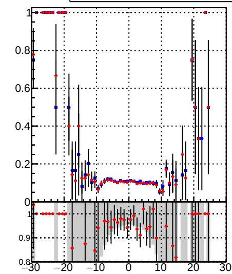
■ DQM_TT_mkFit-DQM_original ■ DQM_TT_mkFit-DQM_modified3
