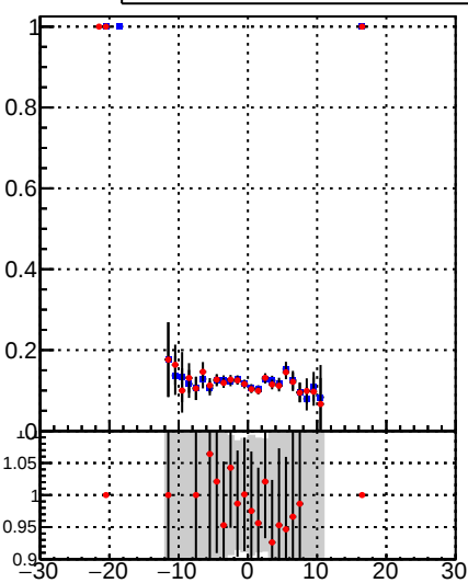
—•— DQM_TT_mkFit-DQM_original —•— DQM_TT_mkFit-DQM_modified3
