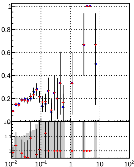
—•— DQM_TT_mkFit-DQM_original —•— DQM_TT_mkFit-DQM_modified3
