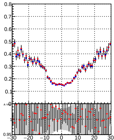
Fake rate vs d —●— DQM_TT_mkFit-DQM_original —●— DQM_TT_mkFit-DQM_modified3
