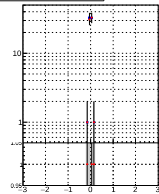
N of associated (recoToSim) tracks vs \eta DQM_TT_mkFit-DQM_original DQM_TT_mkFit-DQM_modified3
