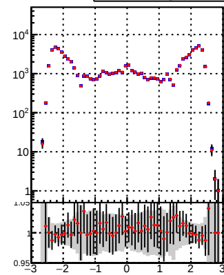
N of reco track vs \eta DQM_TT_mkFit-DQM_original DQM_TT_mkFit-DQM_modified3
