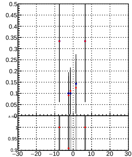
Fake rate vs d —●— DQM_TT_mkFit-DQM_original —●— DQM_TT_mkFit-DQM_modified3
