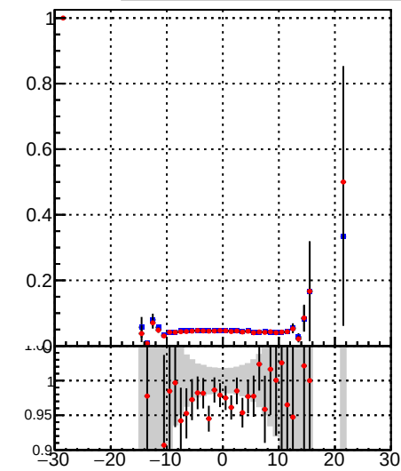
■ DQM_TT_mkFit-DQM_original ● DQM_TT_mkFit-DQM_modified3
