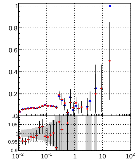
■ DQM_TT_mkFit-DQM_original ● DQM_TT_mkFit-DQM_modified3
