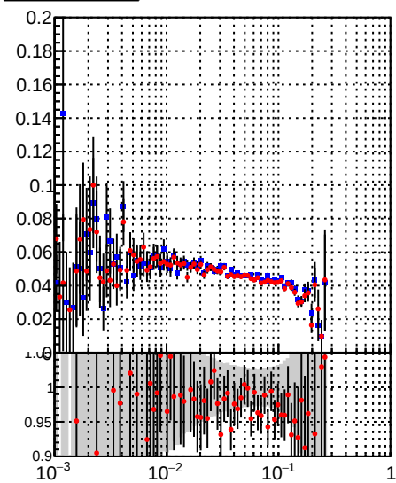
—■— DQM_TT_mkFit-DQM_original —●— DQM_TT_mkFit-DQM_modified3
